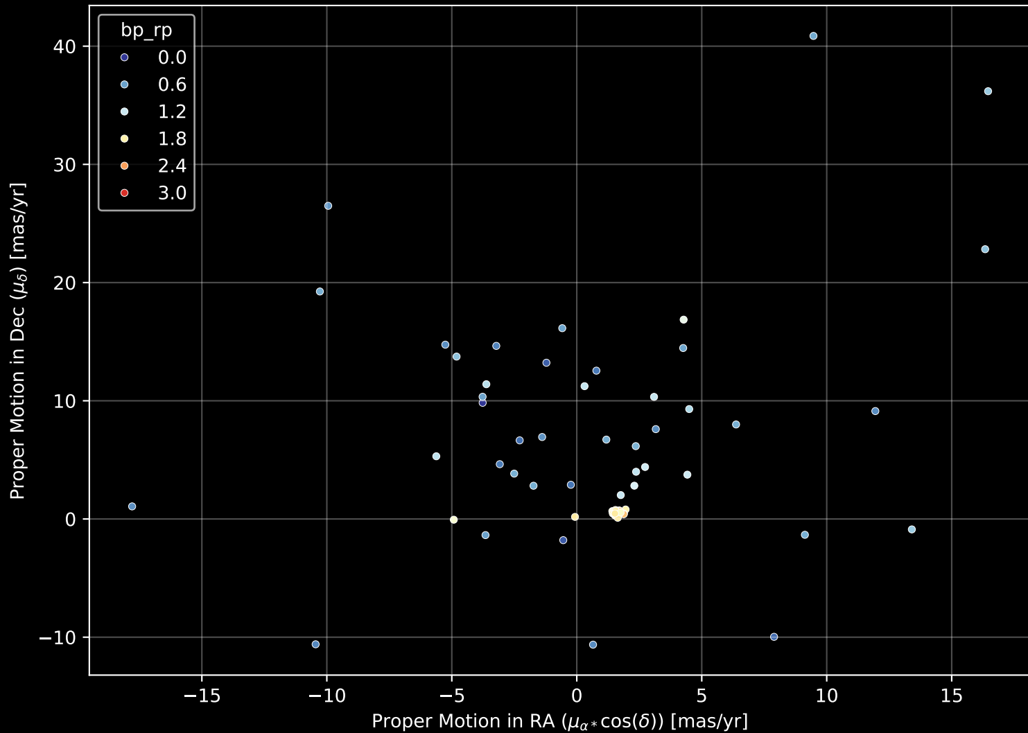
APOGEE DR17 Field: [LMC11] Proper Motion Diagram (n= 104)
