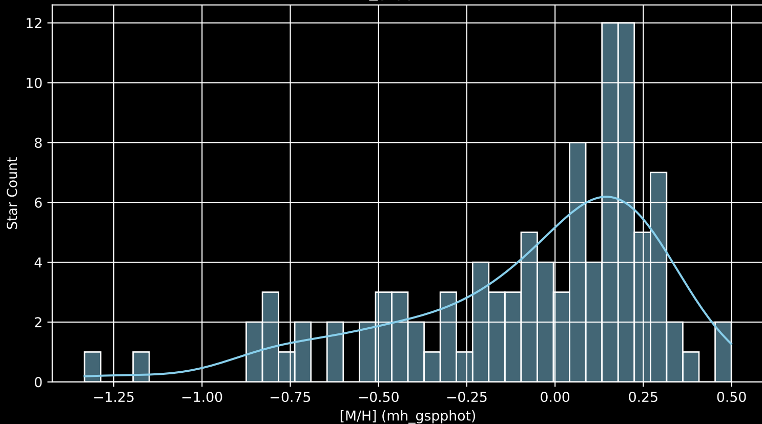
APOGEE DR17 Field: [LMC11 [M/H] (mh_gspphot) (n= 102)
