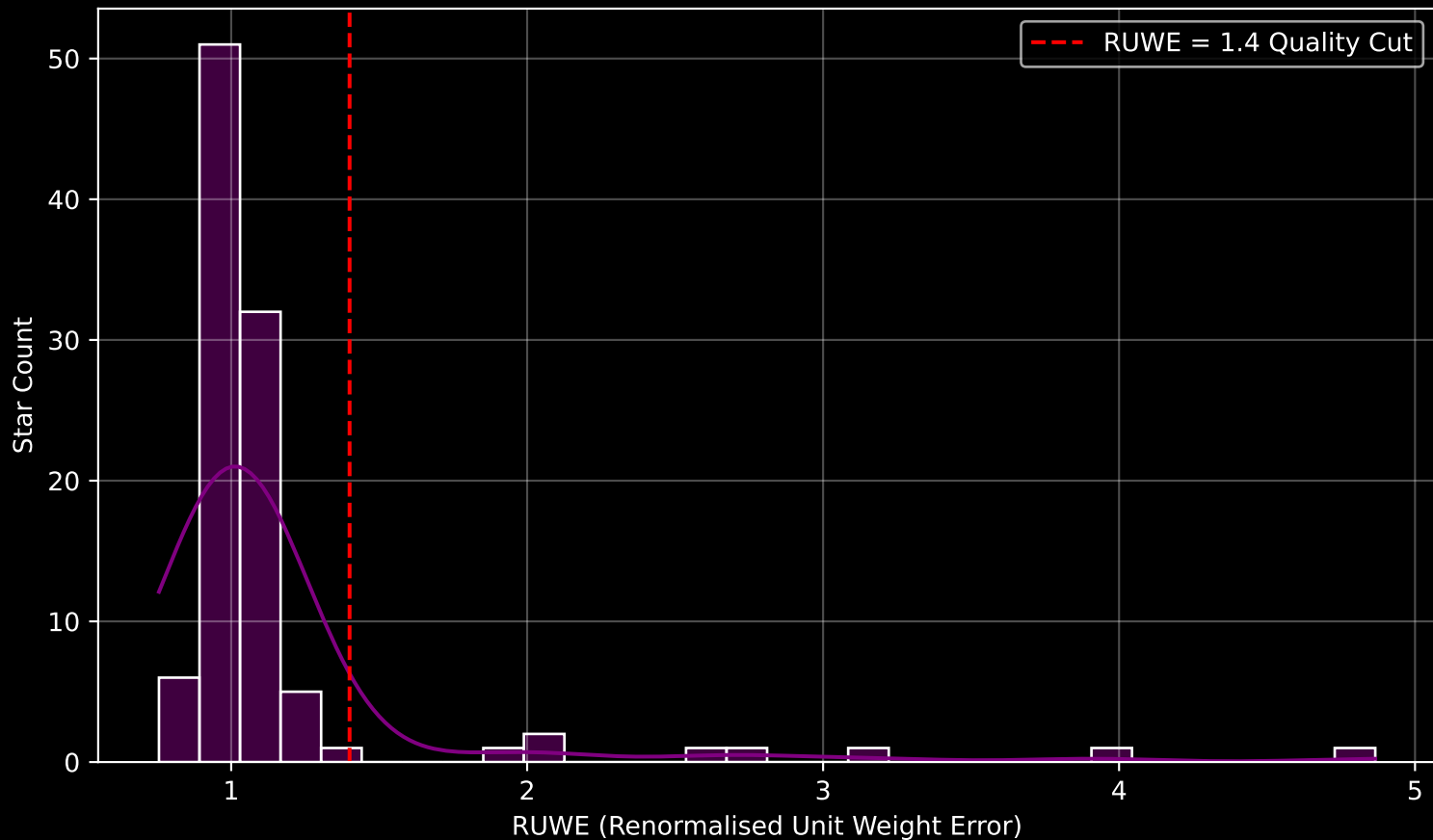
GAPOGEE DR17 Field [LMC11] RUWE Distribution (n= 103)
