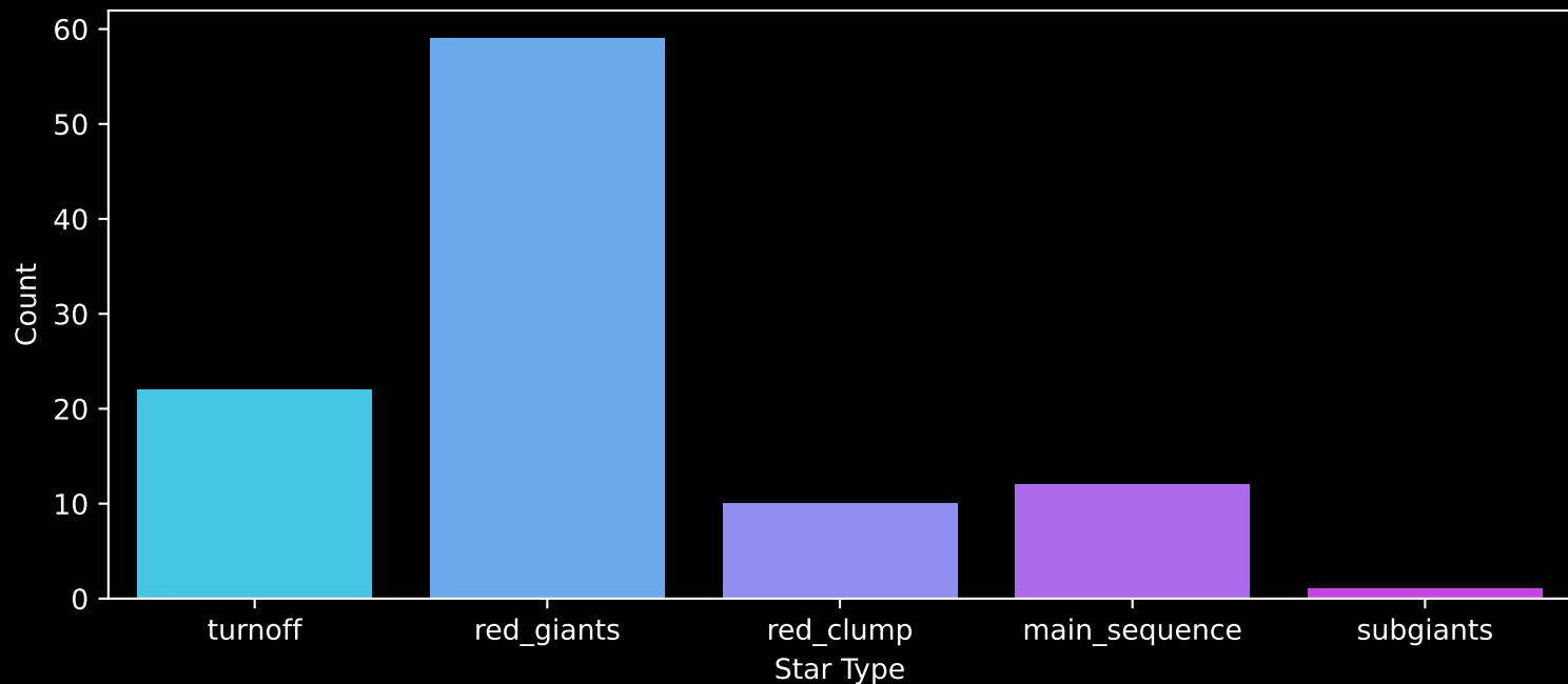
APOGEE DR17 Field: [LMC11] Count plot of Star Type
