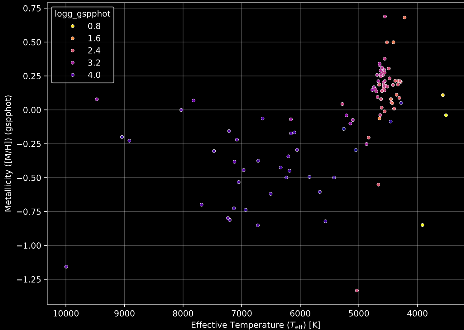
APOGEE DR17 Field: [LMC11] Stellar Population Parameters (n= 104)
