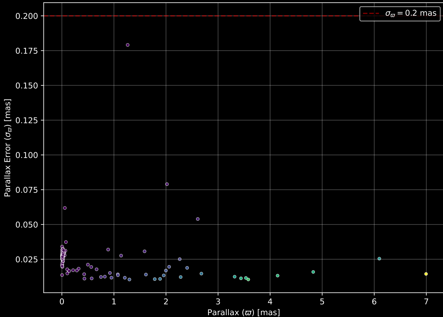
APOGEE DR17 Field: [LMC11] Parallax Quality (n= 104)
